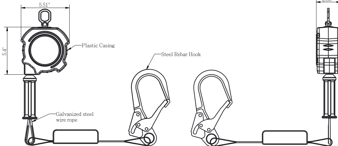
FRONT VIEW SRL411222
