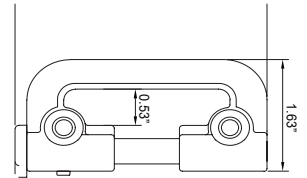
Hook Twin SRL Steel Connector
